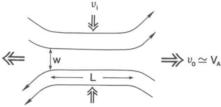
(a) Sweet-Parker reconnection
