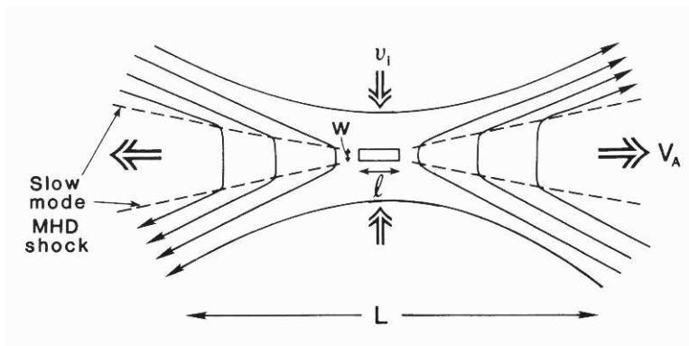
(b) Petschek reconnection
