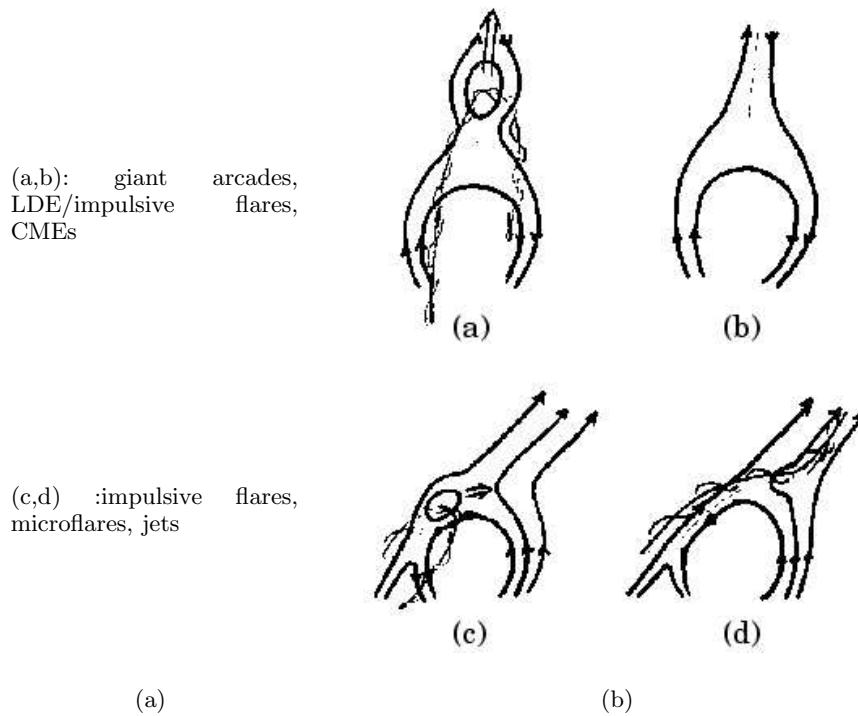
Figure 4. Unified model (Shibata 1999)
