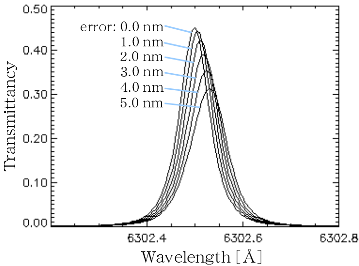
Change of main-peak profile depending on error of thickness of etalon2
