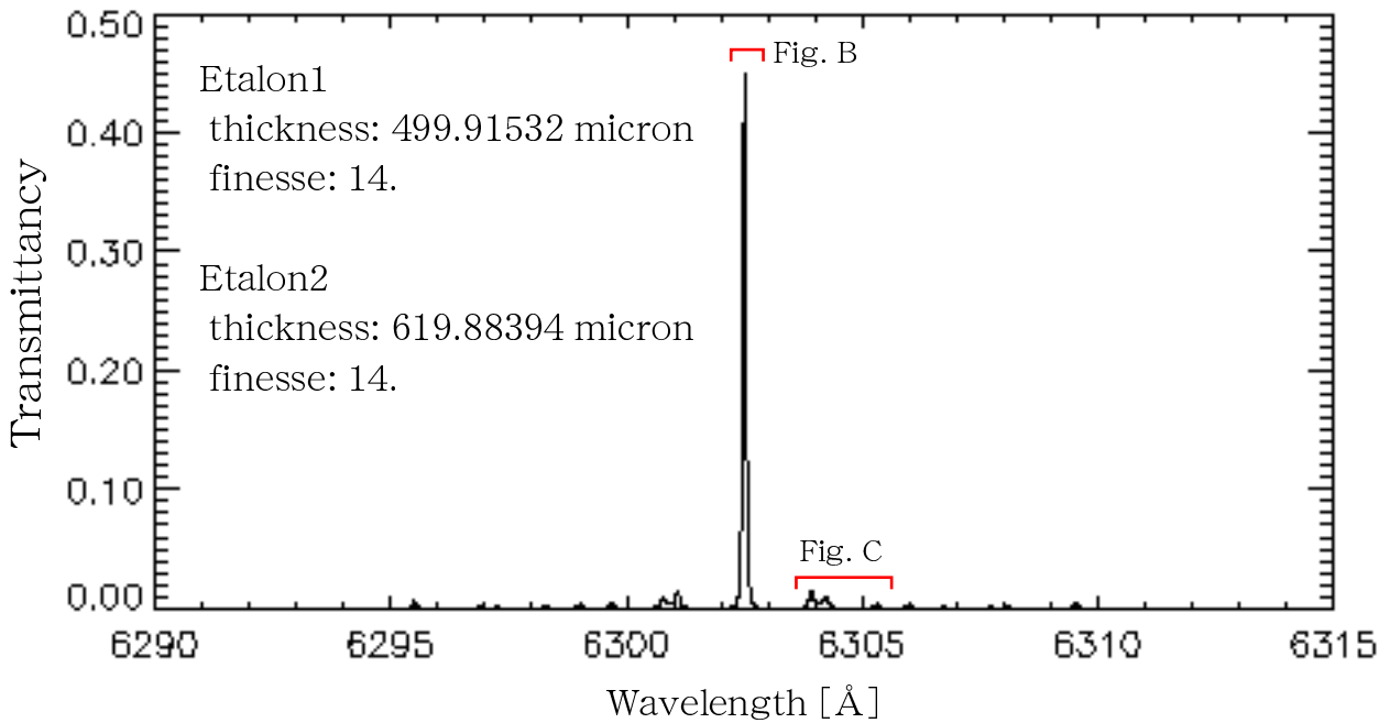
Tandem Fabry-Perot Filter Idealized Profile
