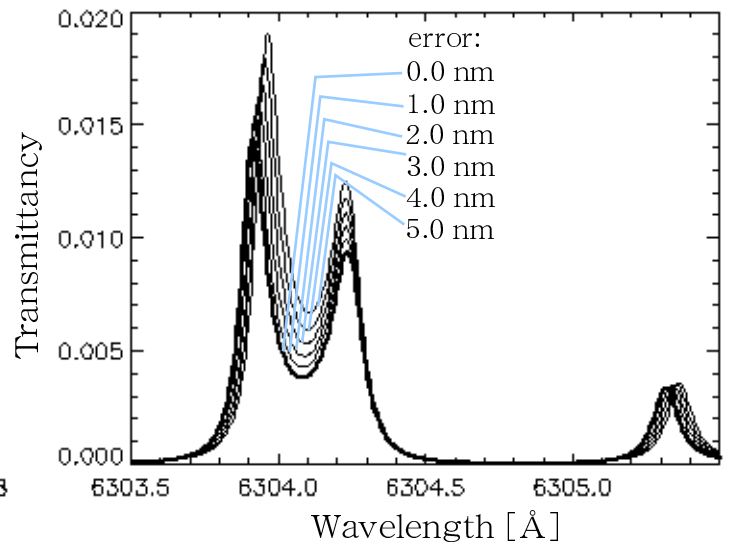
Change of sub-peaks profile depending on error of thickness of etalon2
