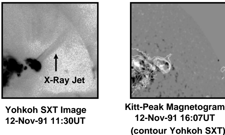
Figure 17: Left: An X-ray jet observed with Yohkoh SXT on 12 Nov. 1991 [154]. Right: NSO/Kitt Peak magnetogram for the same region with overlay contours of the soft X-ray intensity distribution. Note the mixed polarities at the footpoint of the jet.
