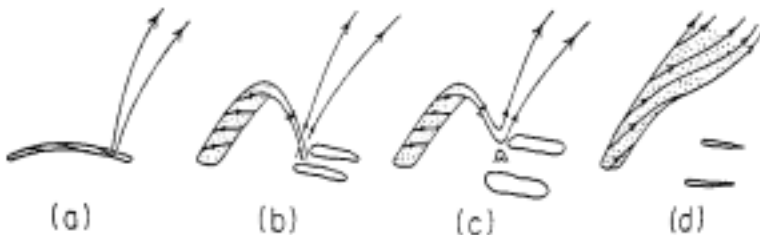
Figure 20: Schematic illustration of the formation of a spinning magnetic-twist jet as a result of reconnection between a twisted flux tube and an untwisted flux tube [151].
